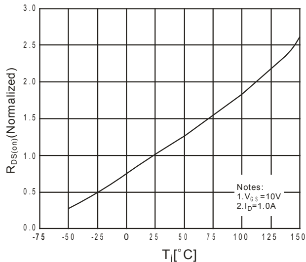
Fig.8 On-Resistance Variation vs. temperature
