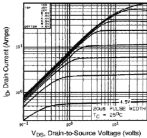
Fig.1 On-State Characteristics
