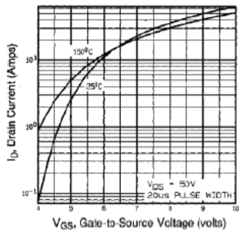
Fig.2 Transfer characteristics
