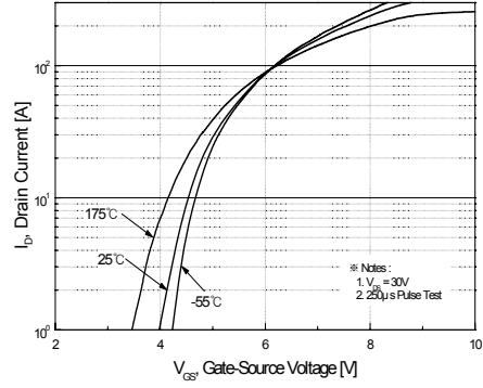
Figure 2. Transfer Characteristics
