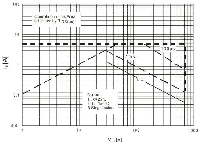
Fig.9 Maximum Safe Operation Area
