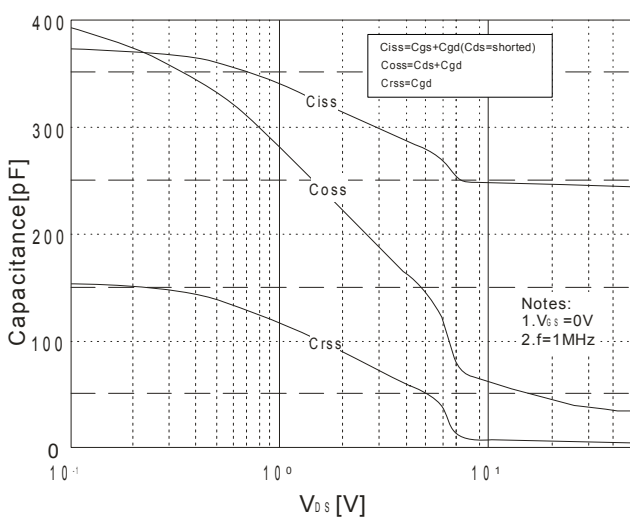
Fig.5 Capacitance characteristics
