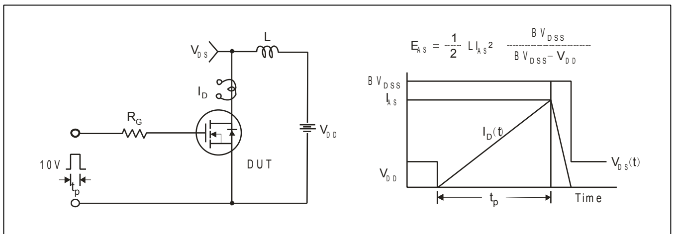
Fig.14 Unclamped Inductive Switching Test Circuit & Waveform
