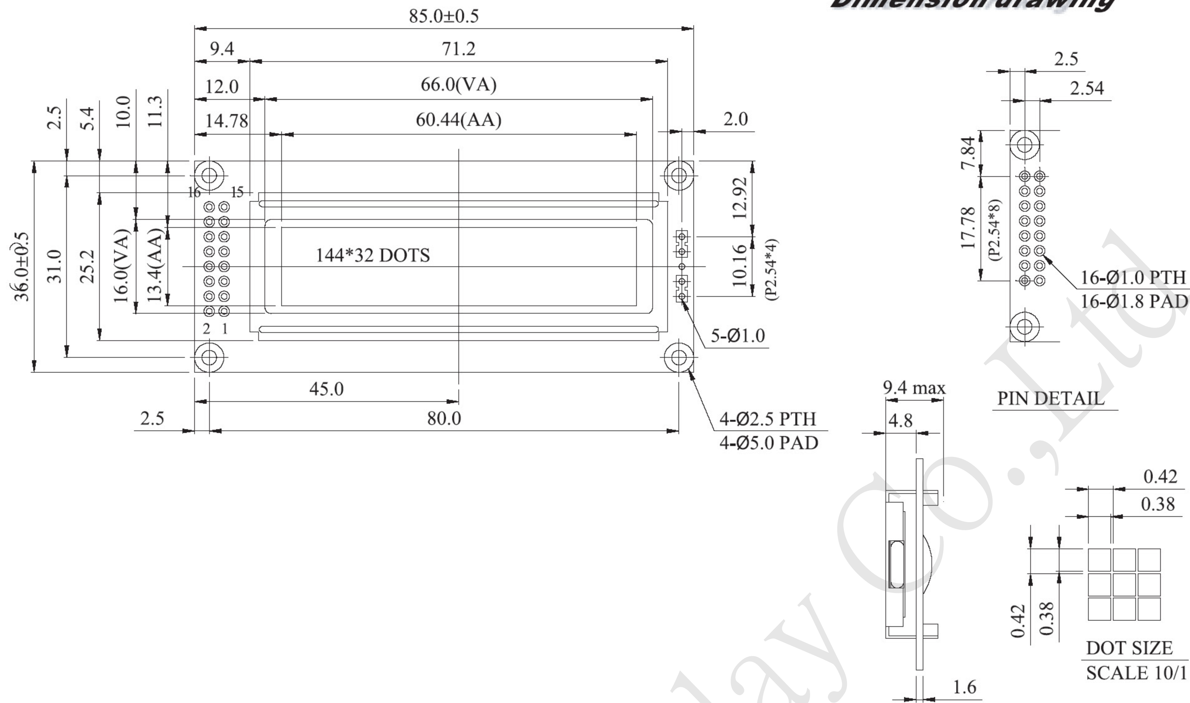
Dimension drawing
