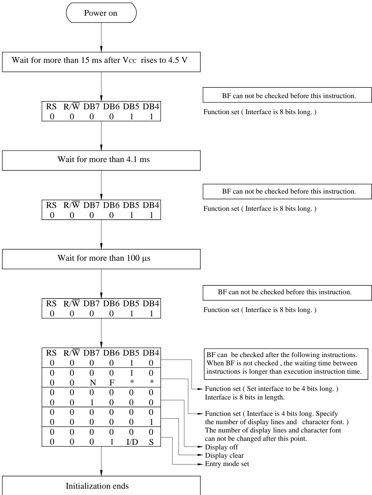
4-Bit Ineterface
