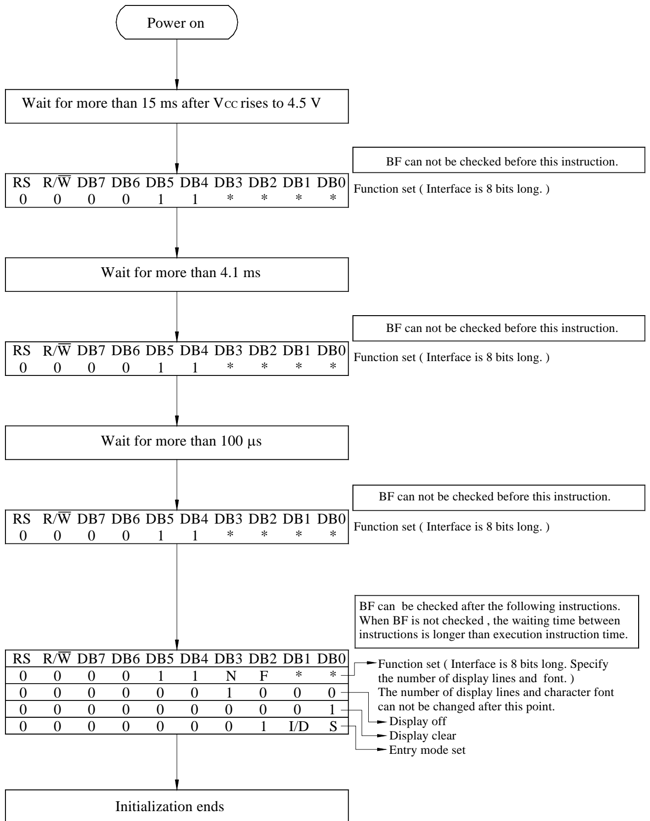
8-Bit Ineterface
