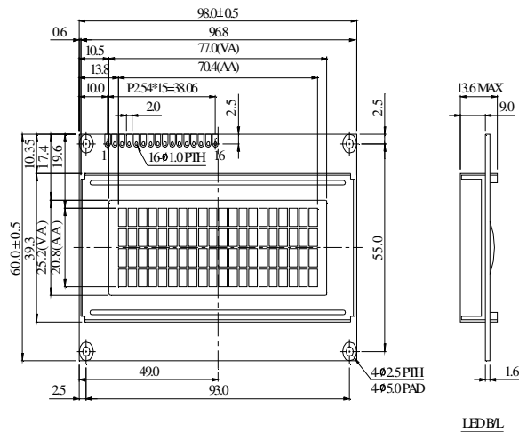
LEDBL
