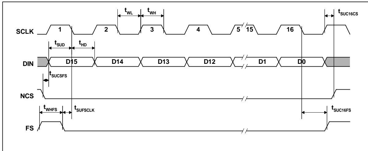
Figure 1 Timing Diagram
