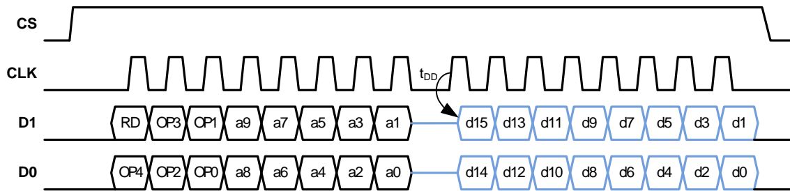
Figure 25. DSPI Read Cycle Detail
