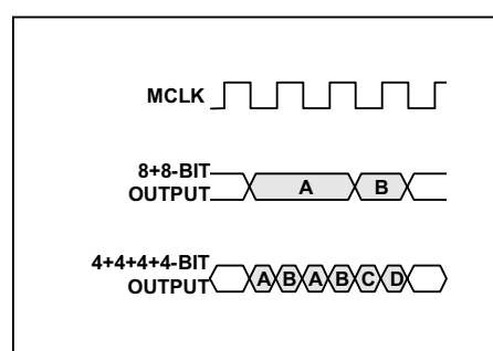
Figure 13 Output Data Formats (Mode 3)
