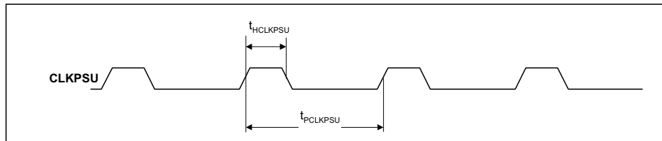
Figure 24 External Power Supply Clock
