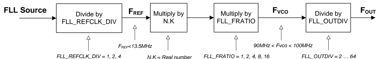
Figure 59 FLL Configuration
