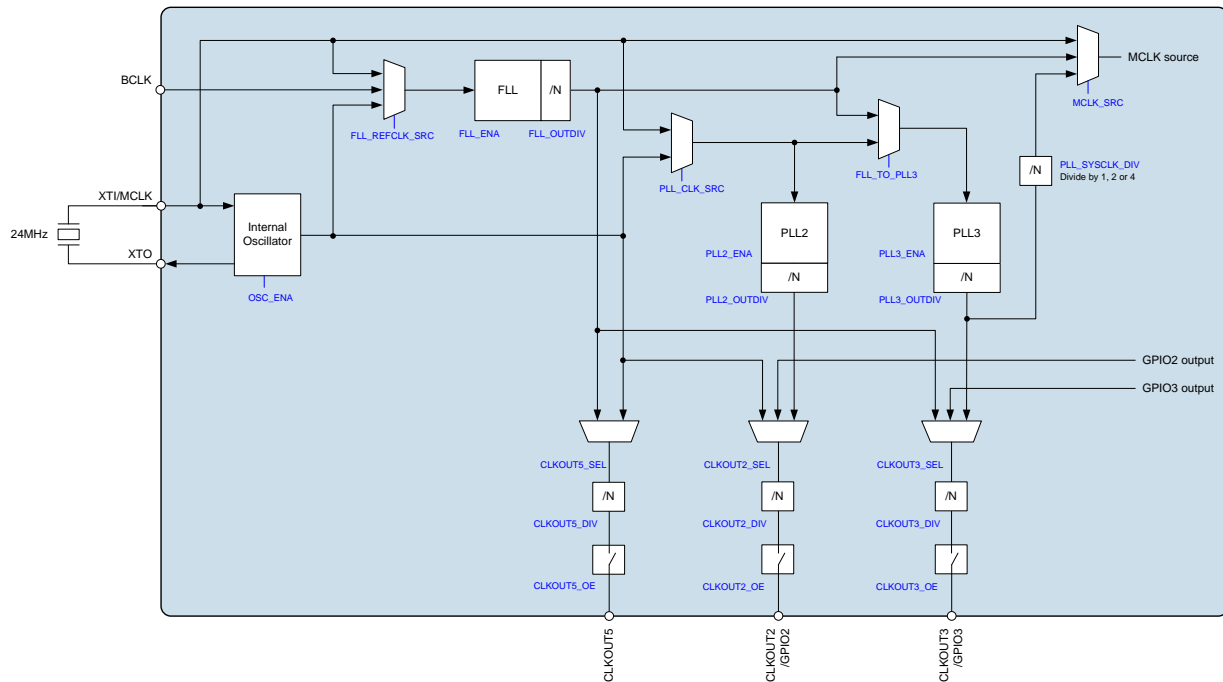
Figure 57 Clock Generation Block Diagram
