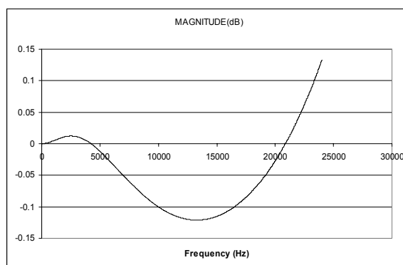
Figure 103 De-Emphasis Error (48kHz)
