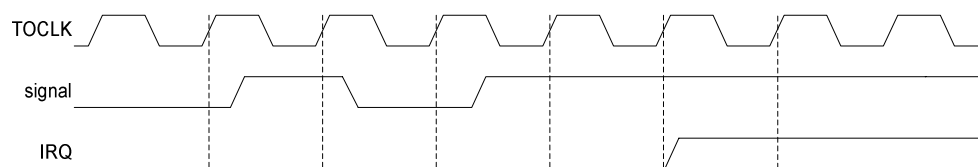
Figure 48 GPIO De-bounce
