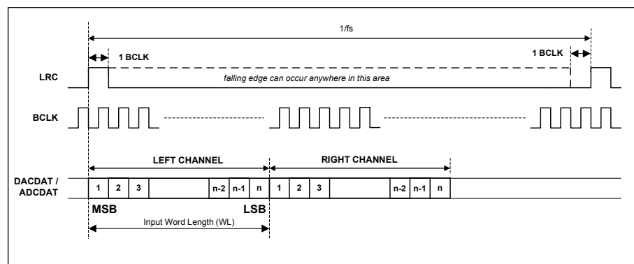
Figure 72 DSP Mode Audio Interface (mode B, AIF_LRCLK_INV=1, Slave)
