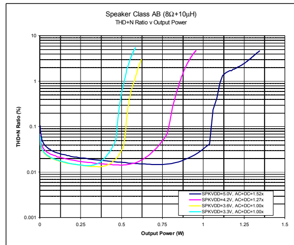
SPEAKER CLASS AB INTO 8\Omega + 10\mu H
