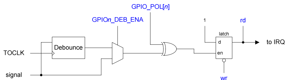
Figure 46 GPIO Function
