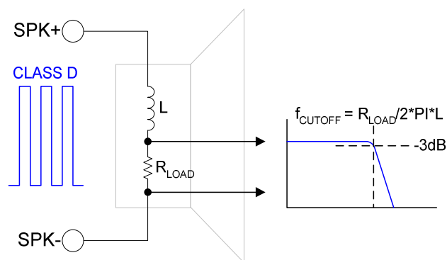
Figure 104 Speaker Equivalent Circuit
