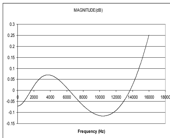
Figure 99 De-Emphasis Error (32kHz)
