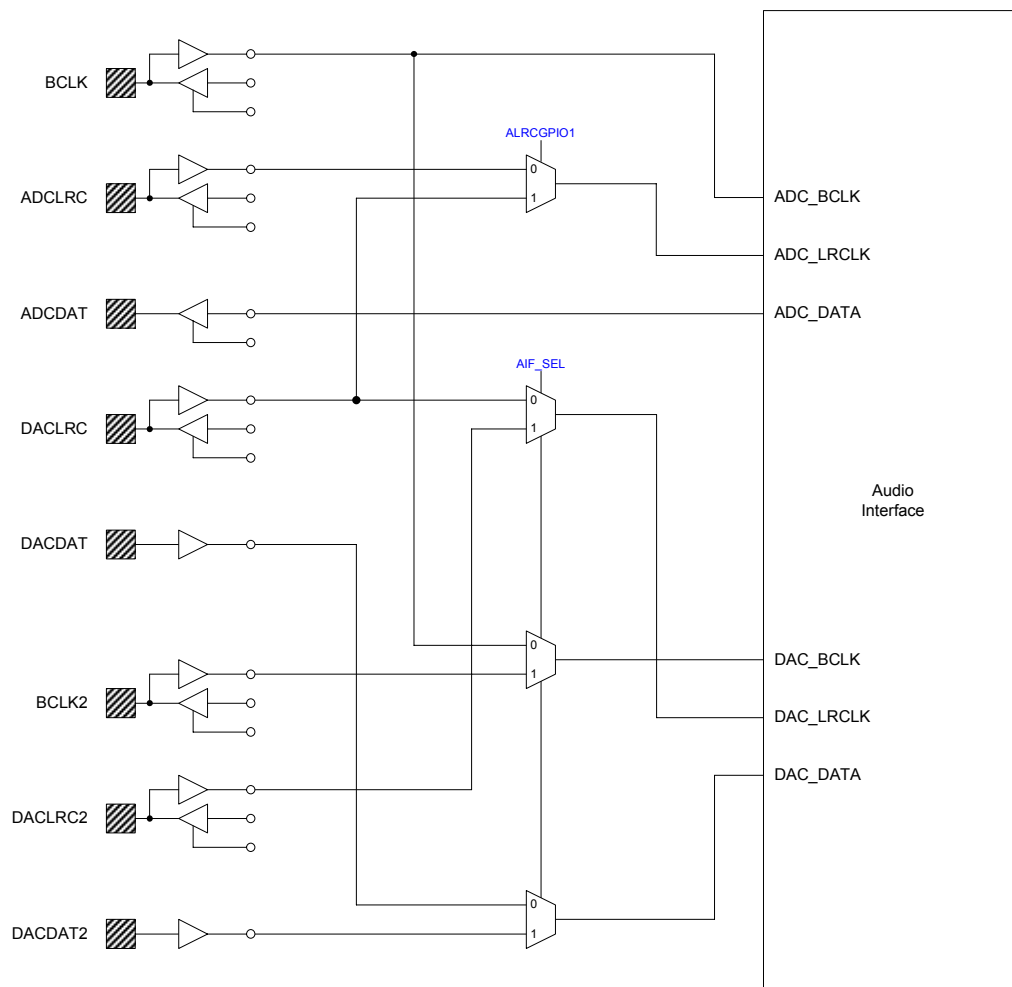
Figure 61 Audio Interface Input Flow
