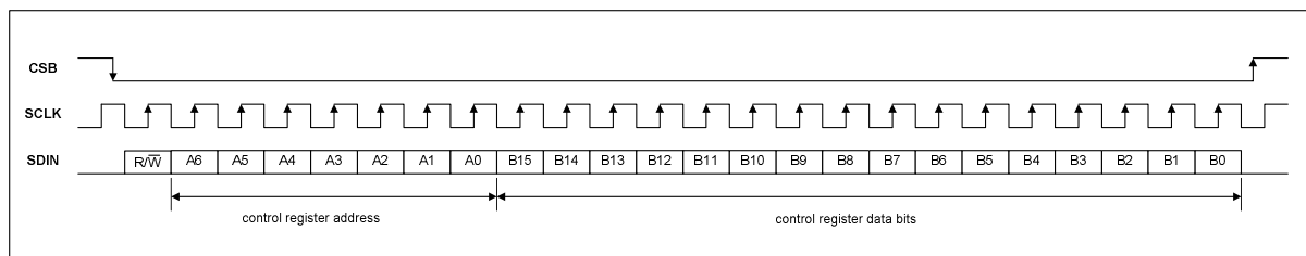
Figure 86 3-Wire Serial Control Interface
