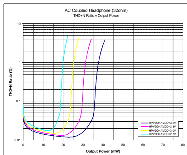
AC COUPLED HEADPHONE INTO 32\Omega
