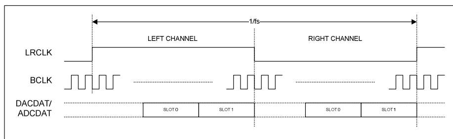
Figure 51 TDM in Right-Justified Mode
