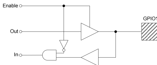
Figure 36 GPIO Pad
