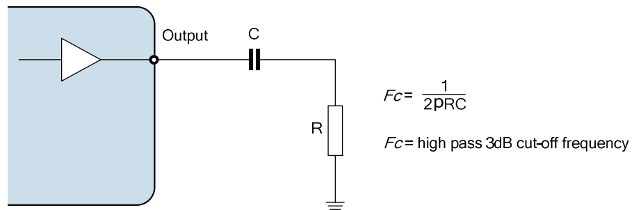
Figure 86 Line Output Path Components
