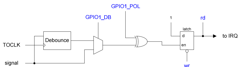
Figure 37 GPIO Function
