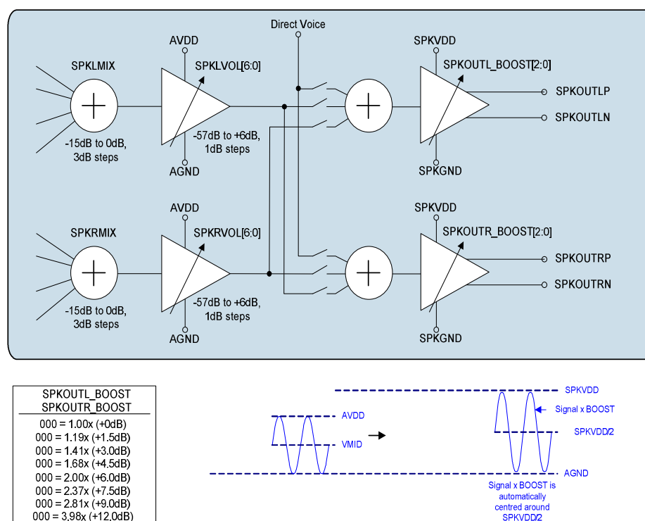
Figure 26 Speaker Output Configuration and AC Boost Operation
