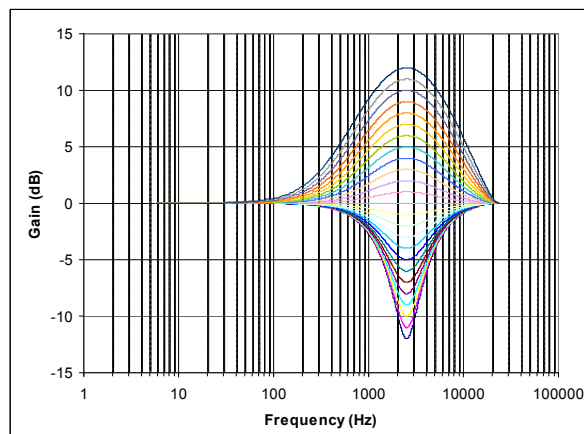
Figure 19 EQ Band 4 – Peak Filter Response
