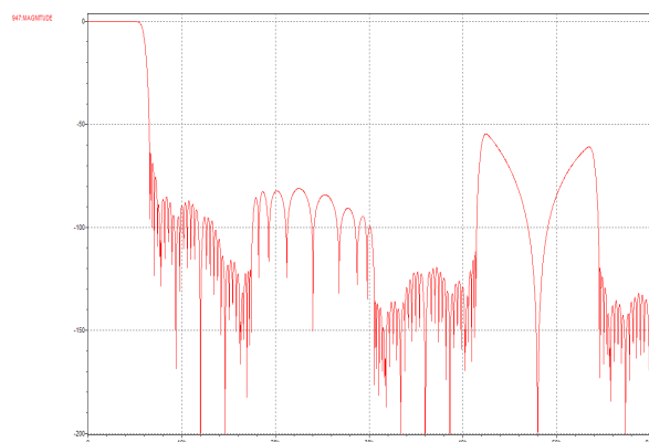
Figure 77 DAC Digital Filter Frequency Response; (Sloping Stopband Mode); Sample Rate \leq 24kHz
