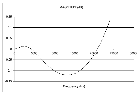
Figure 84 De-Emphasis Error (48kHz)
