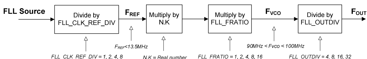
Figure 60 FLL Configuration
