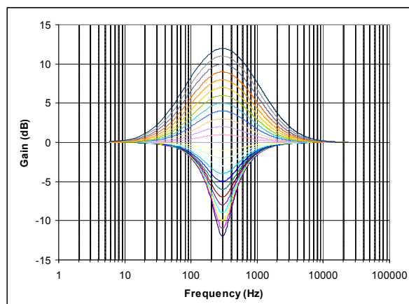
Figure 17 EQ Band 2 – Peak Filter Response
