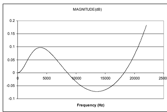
Figure 82 De-Emphasis Error (44.1kHz)
