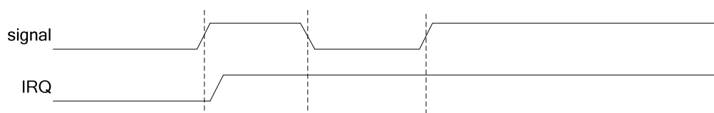
Figure 34 GPIO Latch
