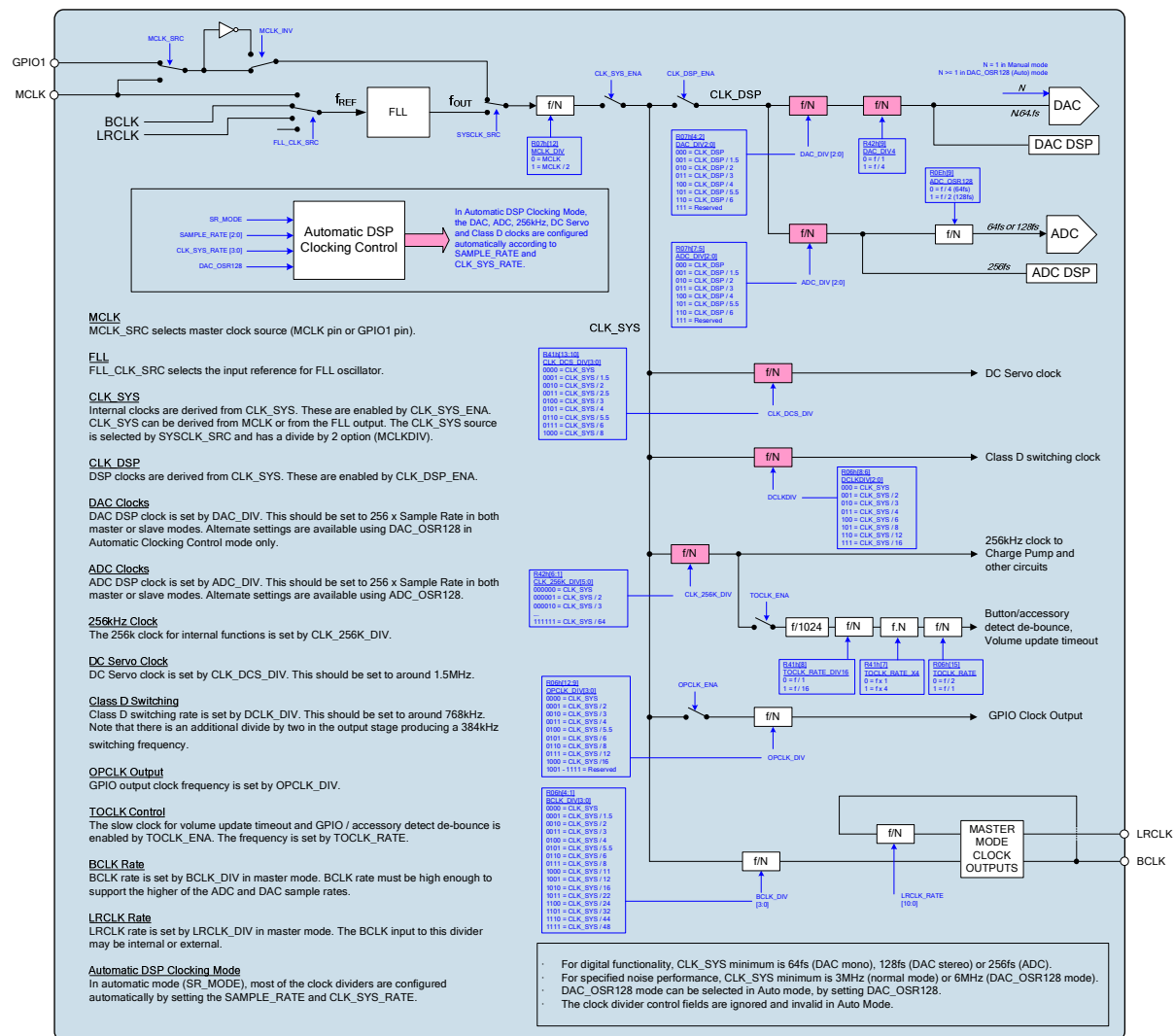
Figure 59 Clocking Scheme
