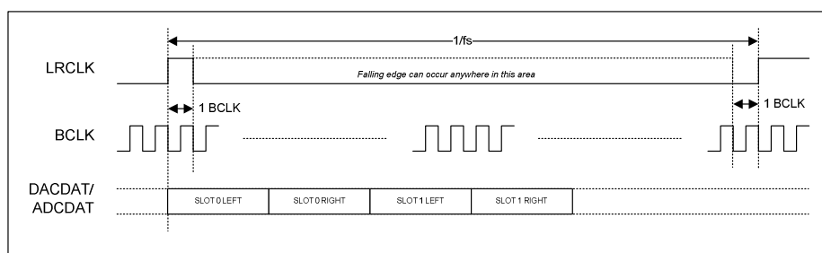
Figure 55 TDM in DSP Mode B
