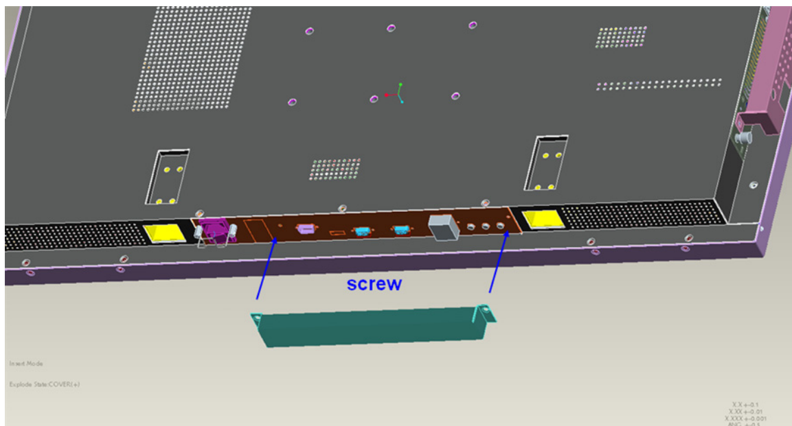
a. Fix cover by fastening 2 screws chassis
