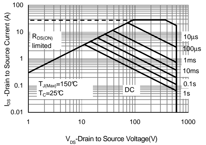
Safe Operating Power (WNM07N65)
