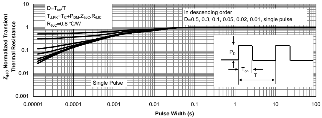
Transient thermal response (Junction-to-Case WNM07N65F)
