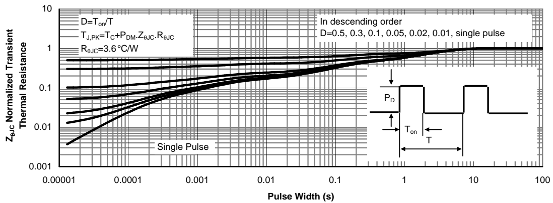
Transient thermal response (Junction-to-Case WNM07N65)
