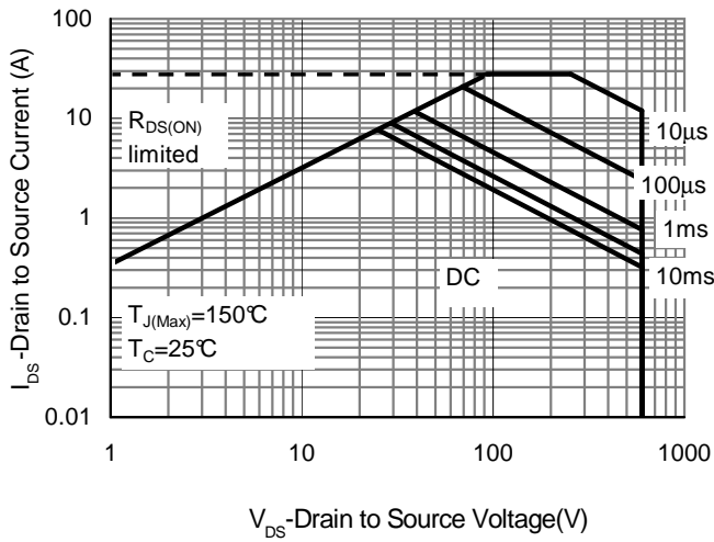
Safe Operating Power (WNM07N65F)
