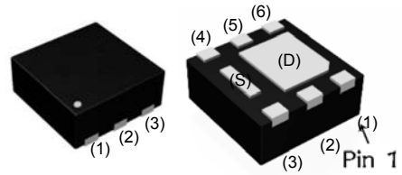
DFN2x2-6L
