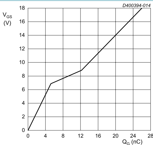
I_{DS} = 2\text{ A} ; I_{GS} = 0.1\text{ mA} ; V_{DS} = 1200\text{ V} ; T_j = 25\text{ }^{\circ}\text{C} Fig. 14. Gate-source voltage as a function of gate charge; typical values
