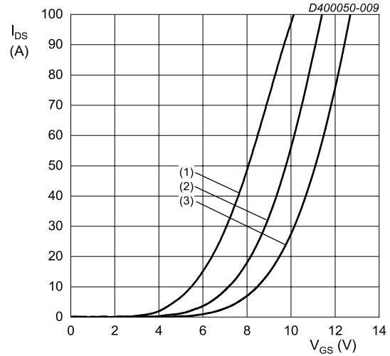
V_{DS} = 20\text{ V}; t_p < 200\ \mu\text{s} (1) T_j = 175\text{ }^\circ\text{C} (2) T_j = 25\text{ }^\circ\text{C} (3) T_j = -55\text{ }^\circ\text{C} Fig. 9. Transfer characteristics; drain current as a function of gate-source voltage; typical values
