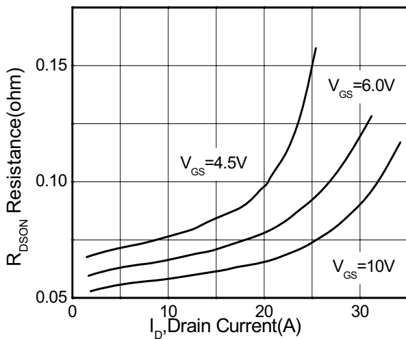
R_{DSON} Resistance VS I_D , Drain Current
