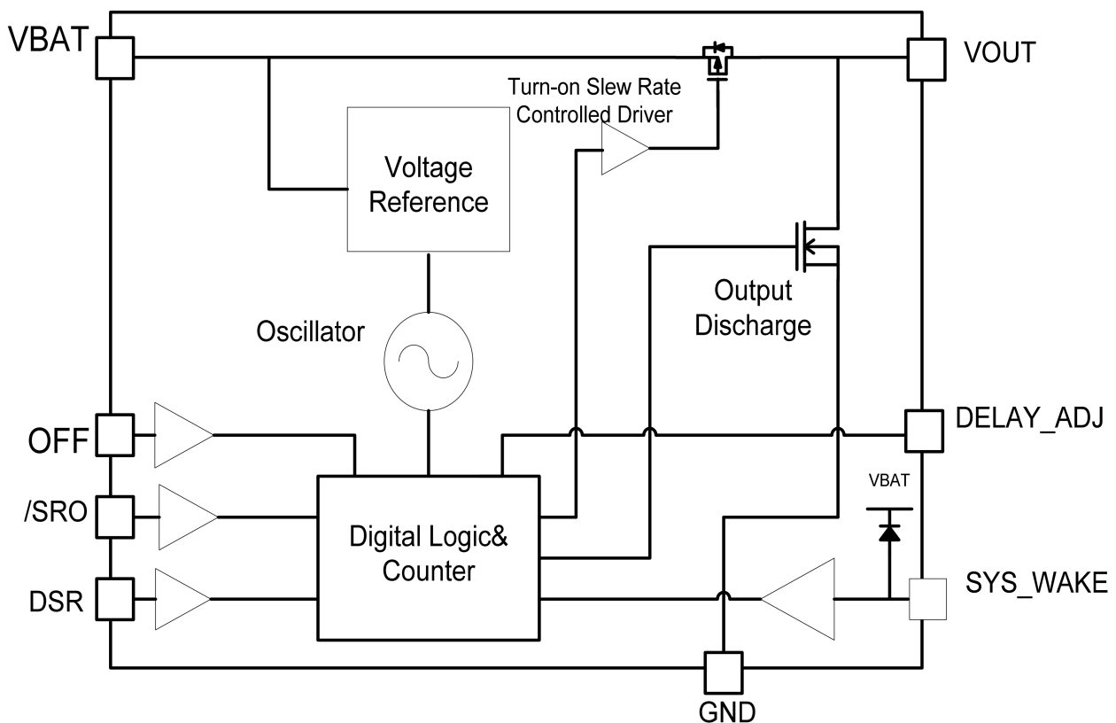
Figure 3. Block Diagram
