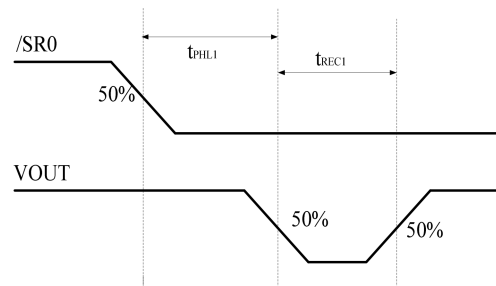
Figure 20. Reset Timing
