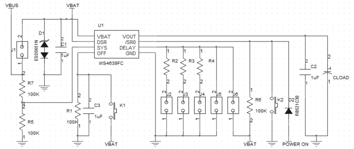
Figure 21. Demo Schematic
