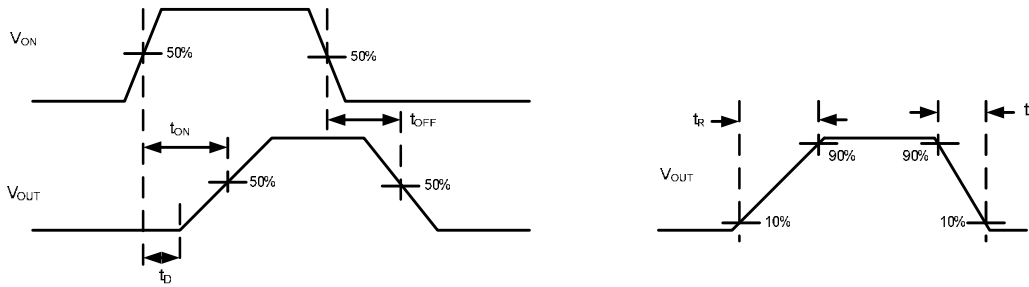
ton/toff WAVEFORMS
