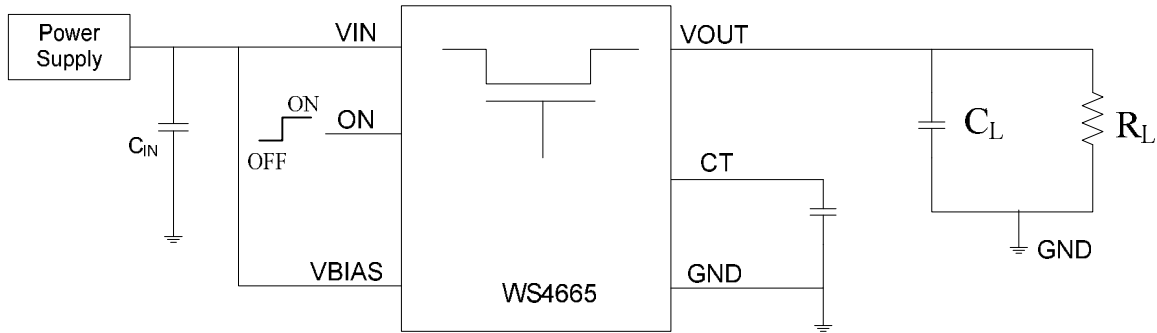
Typical Application
