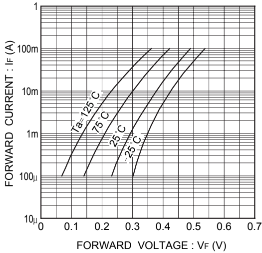
Fig. 1 Forward characteristics
