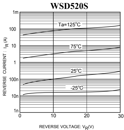
Fig. 2 Reverse characteristics
