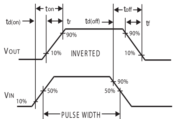
FIG.12 Switching Waveforms
