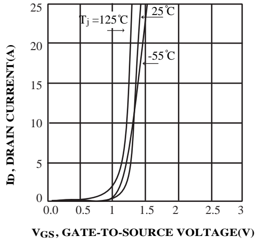
FIG.2 Transfer Characteristics
