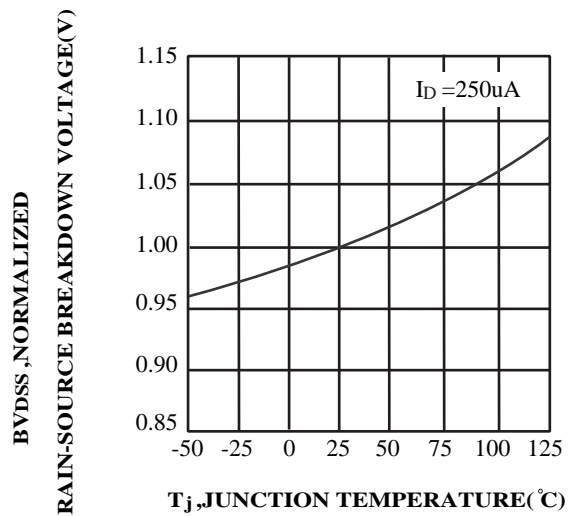
FIG.6 Breakdown Voltage Variation with Temperature
