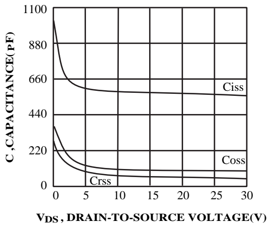
FIG.3 Capacitance
