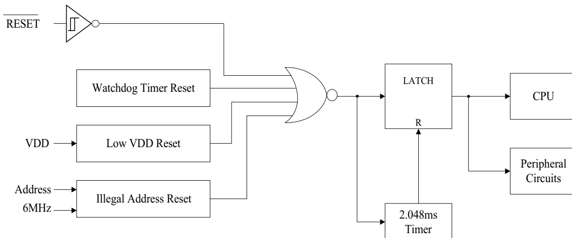
Fig. 1 Reset Signals
