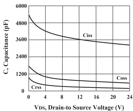
Fig.3 Capacitance
