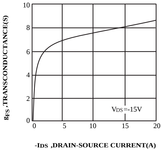
FIG.7 Transconductance Variation with Drain Current
