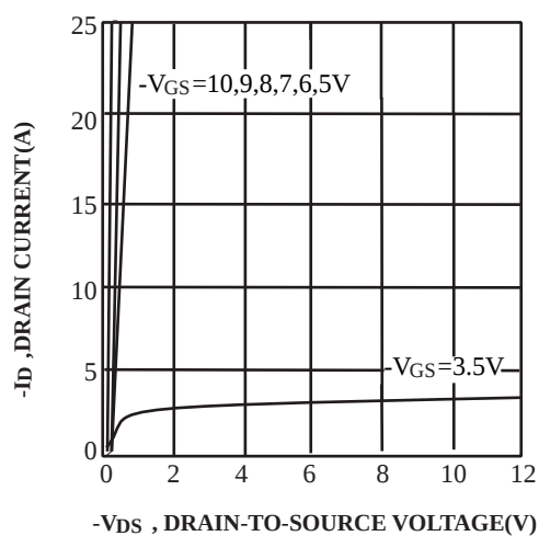
FIG.1. Output Characteristics
