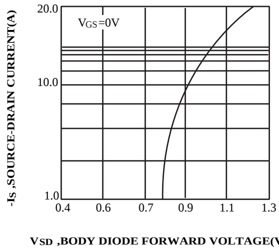
FIG.8 Body Diode Forward Voltage Variation with Source Current
