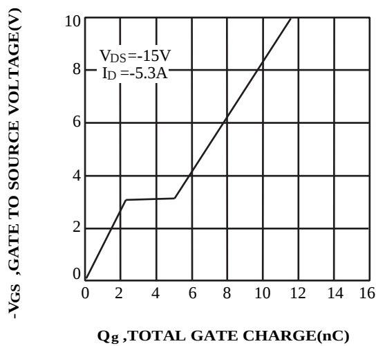
FIG.9 Gate Charge
