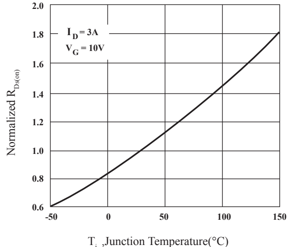
Fig.4 Normalized OnResistance
