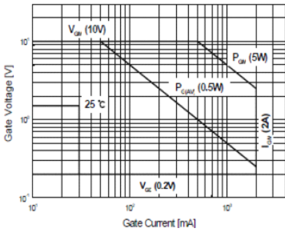
Fig. 3 Gate Characteristics
