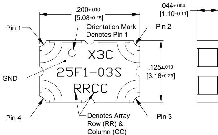
Dimensions are in Inches [Millimeters] X3C25F1-03S Mechanical Outline
