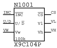
X9C104P N????
