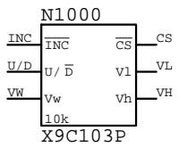
X9C103P N????
