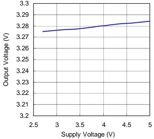
Output Voltage vs. Supply Voltage (IOUT=0A)
