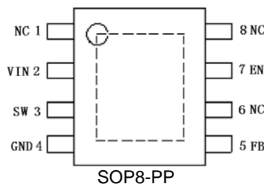
Figure 2. PIN Configuration
