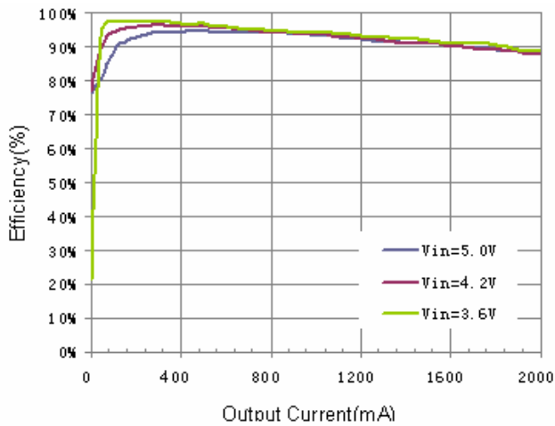
Efficiency vs. Output Current(Vout=3.3V)
