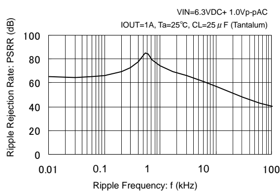
XB1085K12B(VOUT=3.3V)
