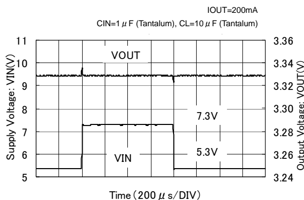
XB1085K12B(VOUT=3.3V)
