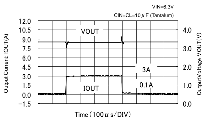
XB1085K12B(VOUT=3.3V)
