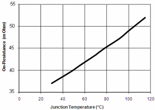
Internal FET On-Resistance vs. Junction Temperature
