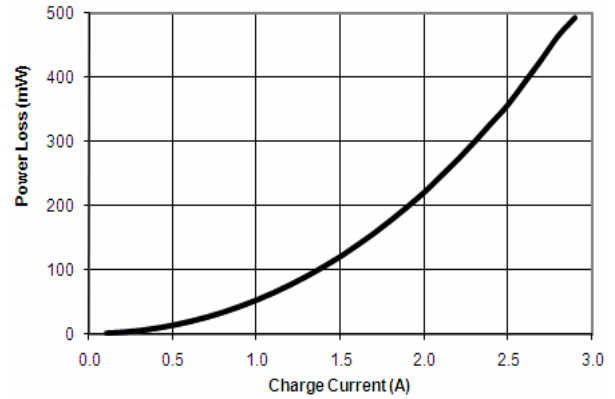
Power Dissipation vs. Charging Current
