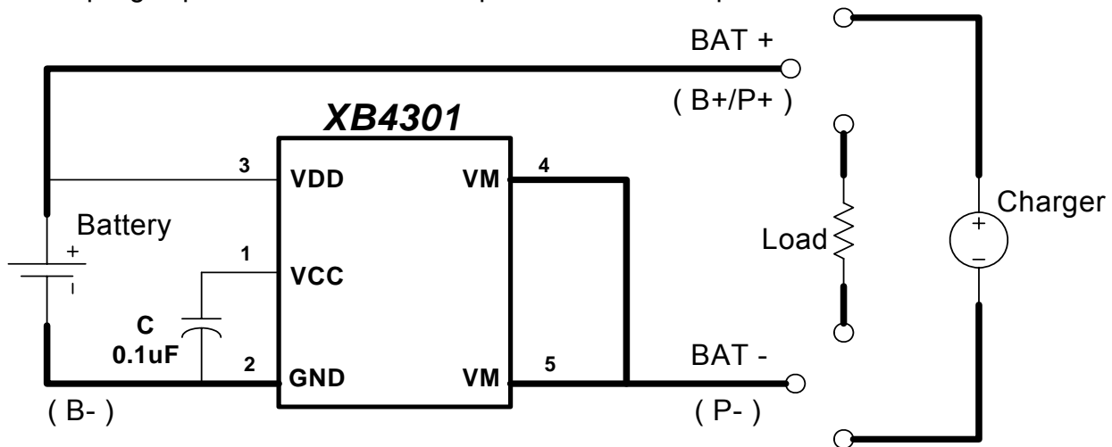
Fig 5 XB301 in a Typical Battery Protection Circuit
