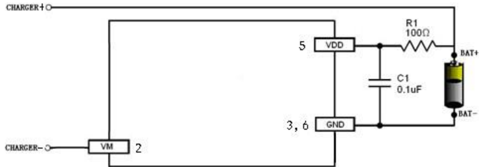
Fig 6 XB5307A in a Typical Battery Protection Circuit
