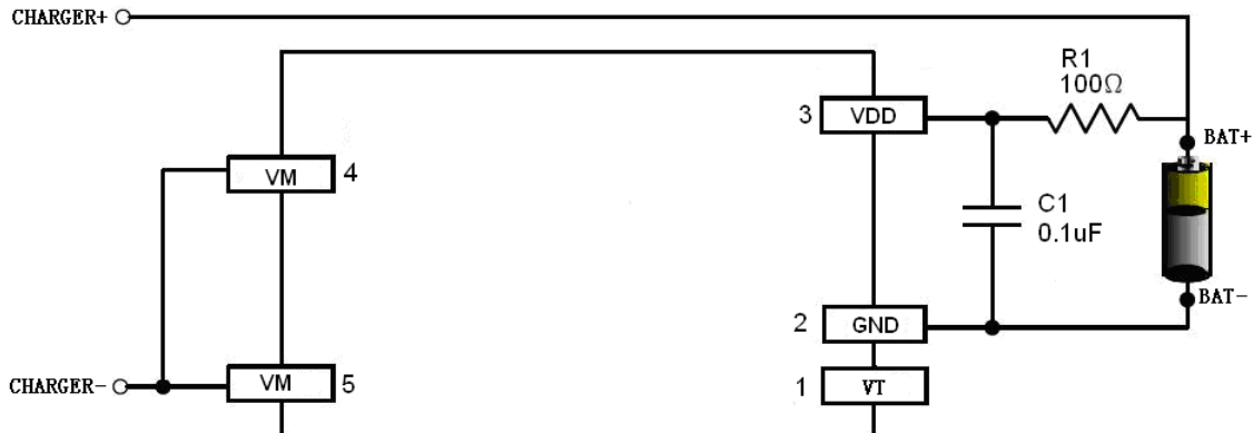
Fig 6 XB5358A in a Typical Battery Protection Circuit
