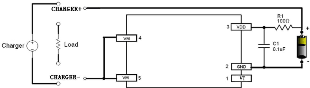
Fig 6 XB5358D0 in a Typical Battery Protection Circuit
