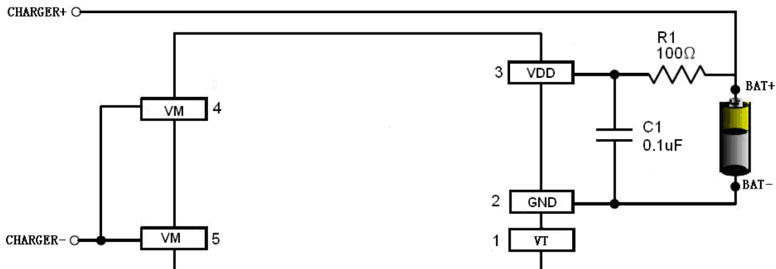
Fig 6 XB5358I0 in a Typical Battery Protection Circuit
