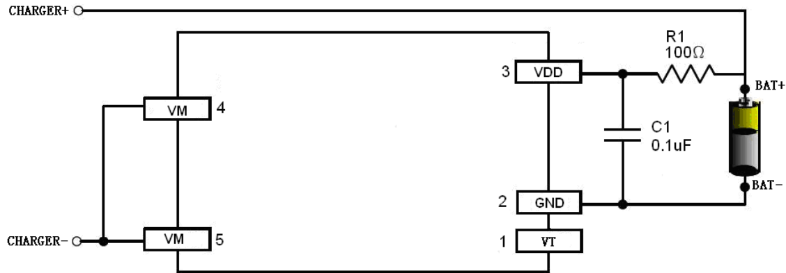
Fig 6 XB5556G in a Typical Battery Protection Circuit
