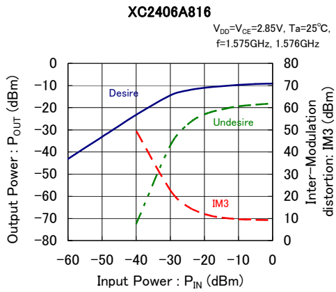
(25) Output Power / IM3 vs. Input Power
