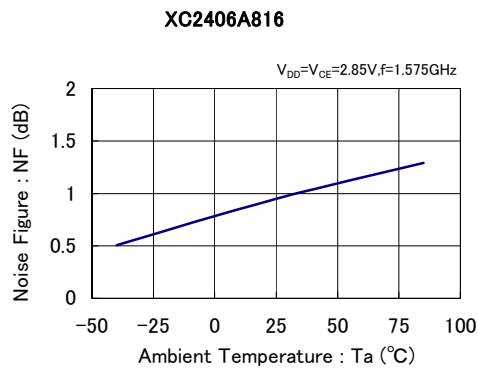
(16) Noise Figure vs. Ambient Temperature
