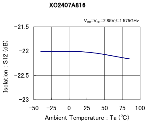
(15) Isolation vs. Ambient Temperature
