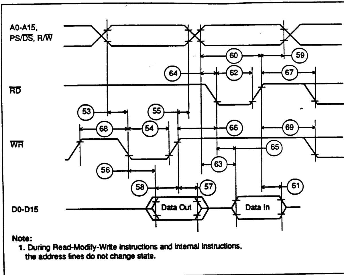
Async. External Bus Figure 1. External Bus Asynchronous Timing
