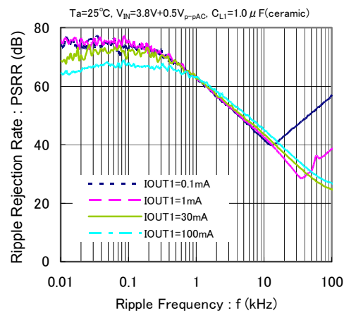
XC6419( V_{OUT1}=2.8V ) VR1
