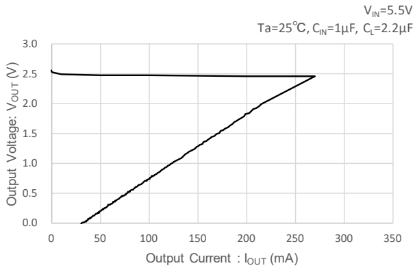
(7-1) V_{OUT(T)}=2.5V
