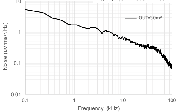
(15-1) XC6706A331P ( V_{OUT(T)}=3.3V )
