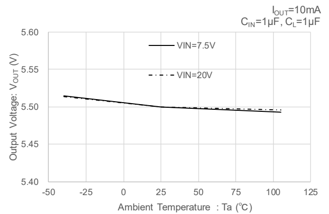
(5-3) V_{OUT(T)}=5.5V
