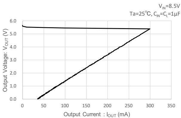
(7-3) V_{OUT(T)}=5.5V
