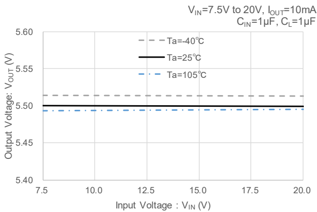
(4-3) V_{OUT(T)}=5.5V
