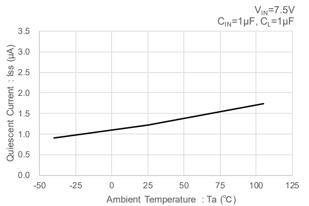
(2-3) V_{OUT(T)}=5.5V
