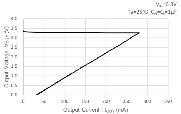
(7-2) V_{OUT(T)}=3.3V
