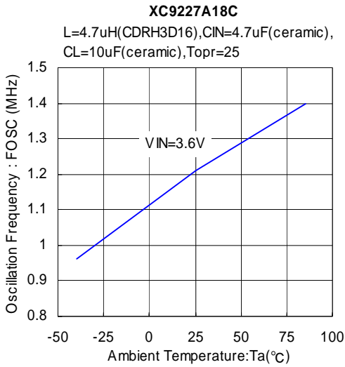
(4) Oscillation Frequency vs. Ambient Temperature
