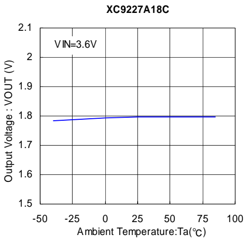
(6) Output Voltage vs. Ambient Temperature
