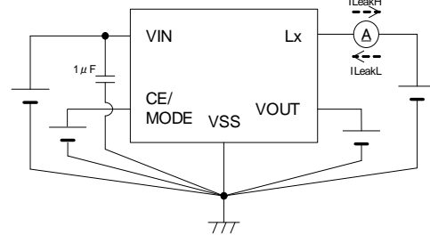
Circuit⑥
