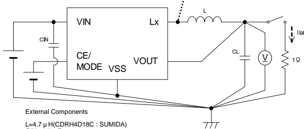
Circuit⑨
