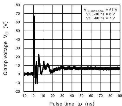
Fig. 11.2.5 ISO10605 Clamp Waveform +8 kV
