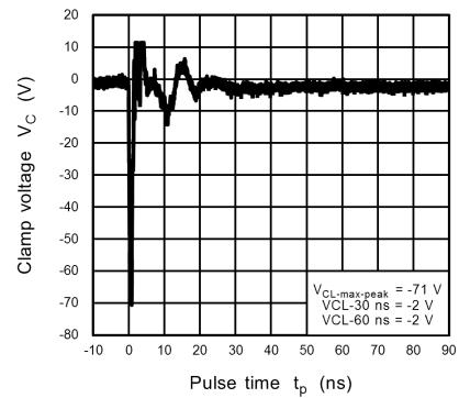
Fig. 11.14.6 ISO10605 Clamp Waveform -8 kV
