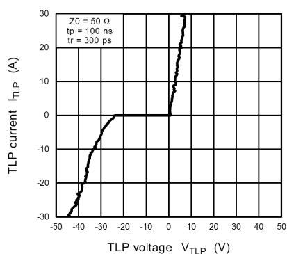
Fig. 11.17.1 I_{TLP} - V_{TLP}
