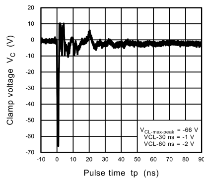
Fig. 11.3.6 ISO10605 Clamp Waveform -8 kV
