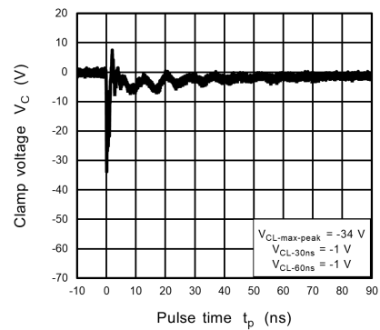
Fig. 11.14.4 IEC61000-4-2 Clamp Waveform -8 kV
