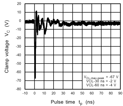
Fig. 11.15.6 ISO10605 Clamp Waveform -8 kV
