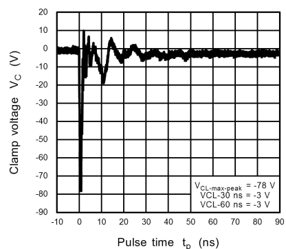
Fig. 11.21.6 ISO10605 Clamp Waveform -8 kV
