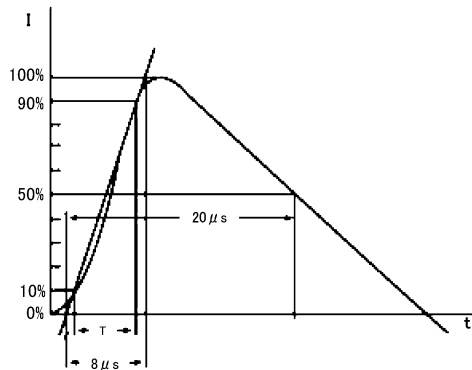
Fig. 11.22.1 V_C - I_{PP} Peak Pulse Current (according to IEC61000-4-5 8/20 \mu s pulse)
