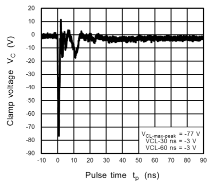
Fig. 11.20.6 ISO10605 Clamp Waveform -8 kV
