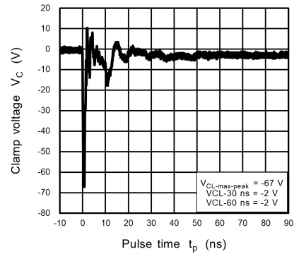
Fig. 11.7.6 ISO10605 Clamp Waveform -8 kV
