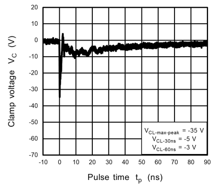
Fig. 11.15.4 IEC61000-4-2 Clamp Waveform -8 kV
