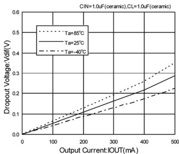
XC6210 (VOUT:2.5V)
